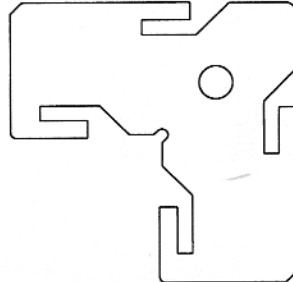
TA-24 Aluminum Casing Corner Piece Finishes: Browntone, Black. Used to ensure tight miters. (used with TA-23, TA-28) See page T-1
