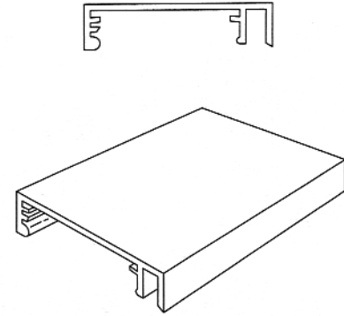
TA-28 Aluminum Casing (1 25/32" Profile) Finishes: Browntone, Black, Alodine. (Consult factory for additional finishes) Only available with 4 1/2" hinge emboss See page T-2
