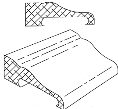
TA-35 Colonial PVC Casing (1 15/16" Profile) Finishes: Navajo White, Browntone, Black, Western White, Autumn Brown, Stone Gray, Winter White. (Consult factory for availability) Not Available on Mullions or Sill See page T-3
