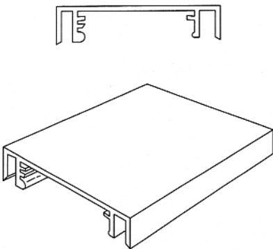
TA-28M Aluminum Mullion Casing (2" Profile) Finishes: Browntone, Black, Alodine. (Consult factory for additional finishes) See page T-2
